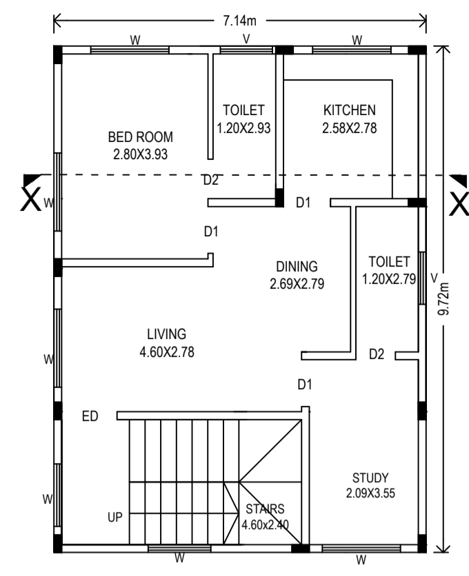
ADDITION AND ALTERATION TO THE EXISTING GROUND FLOOR PLAN
