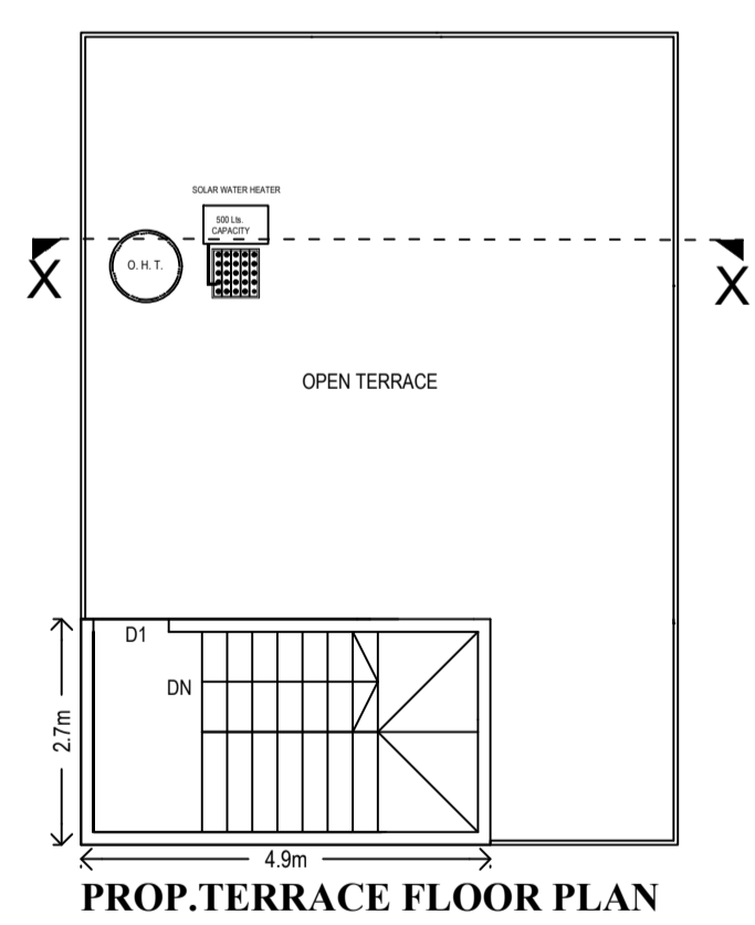
PROP. TERRACE FLOOR PLAN
