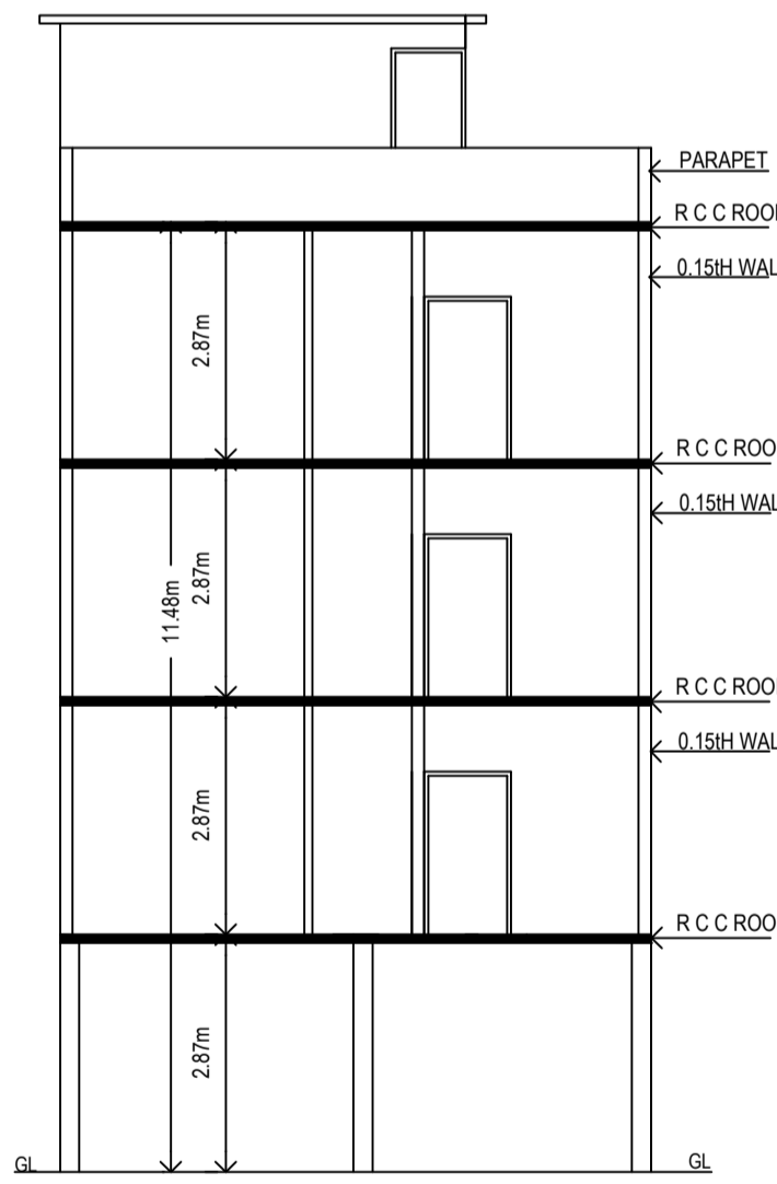
SECTION @ X-X
